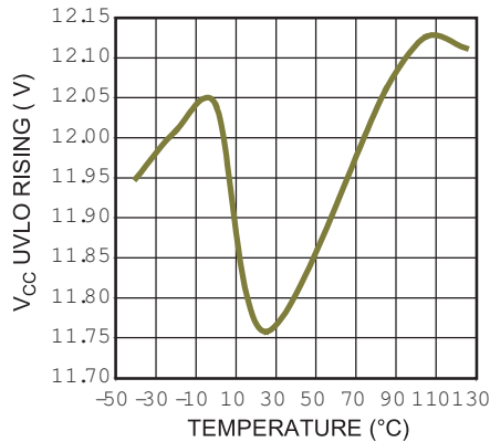
V CC UVLO Rising Threshold vs. Temperature
