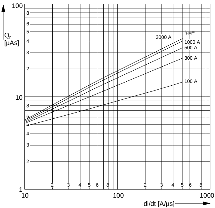
Fig. 4 Reverse recovery charge (upper limit, ca. 98% values) Parameter: I_{FM}
