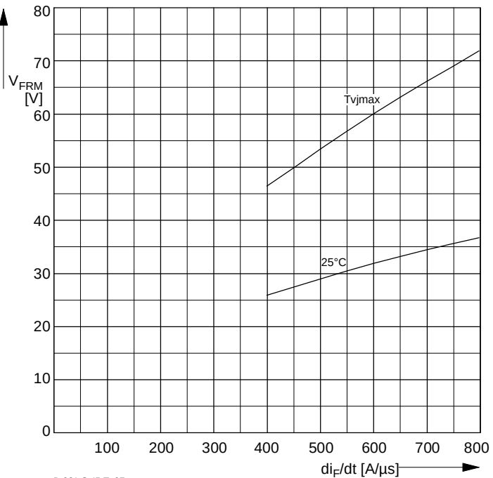
Fig. 7 Peak Forward Recovery Voltage (typical values) Parameter: t_{vj}
