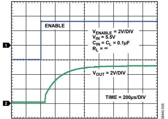
Figure 26. ADR3450 Restart Response from Shutdown
