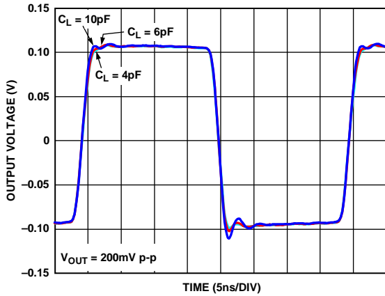
Figure 22. Small Signal Transient Response vs. Capacitive Load
