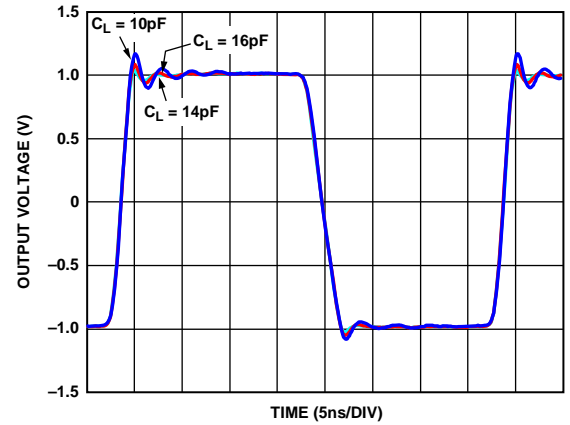
Figure 25. Large Signal Transient Response vs. Capacitive Load
