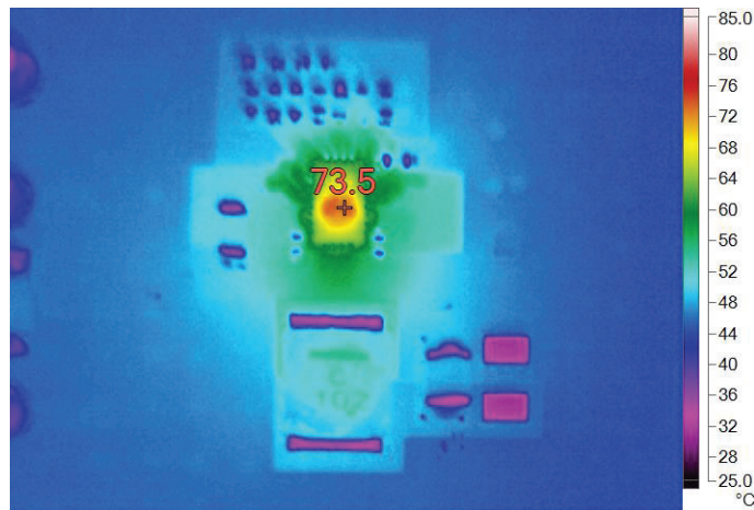
Figure 5. Thermal at 12V IN , 3.3V OUT and 5A OUT , 0LFM
