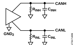
Figure 22. Input Resistance ( R_{INX} ) and Input Capacitance ( C_{INX} ) Measured in Recessive State, Bus Disconnected
