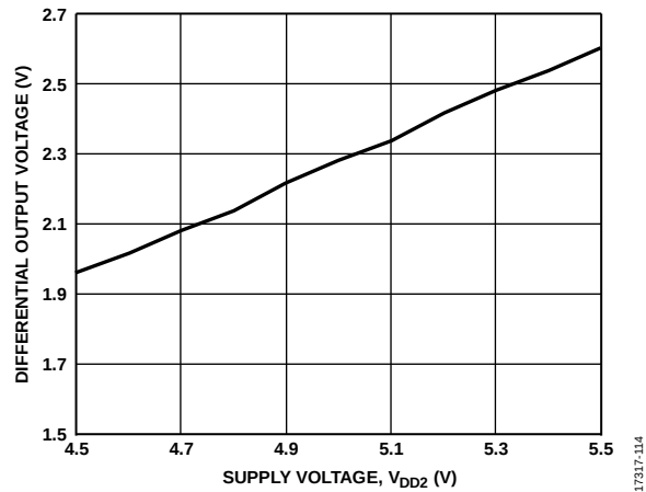
Figure 14. Differential Output Voltage vs. Supply Voltage ( V_{\text{DD2}} ), R_L = 60\ \Omega
