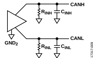
Figure 22. Input Resistance ( R_{IN} ) and Input Capacitance ( C_{IN} ) Measured in Recessive State, Bus Disconnected
