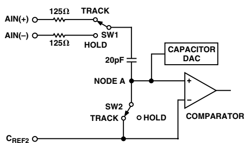
Figure 11. Analog Input Equivalent Circuit
