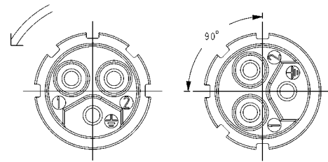
Female / Buchse / Femelle
