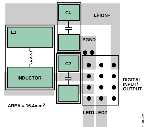
Figure 2. PCB Layout
