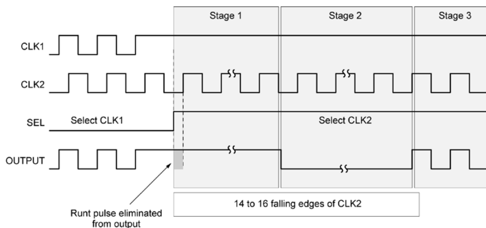
Timing Diagram 2
