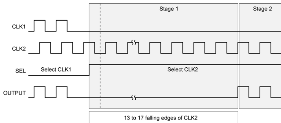
Timing Diagram 3
