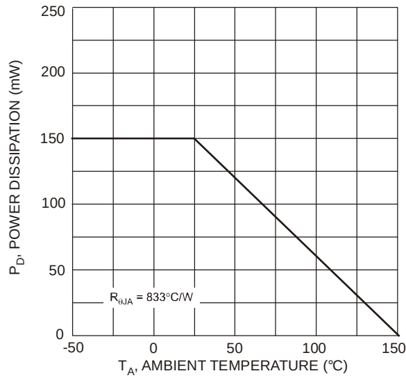
Fig.7 Derating Curve
