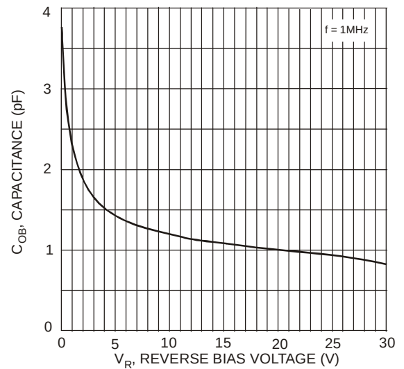
Fig.10 Output Capacitance
