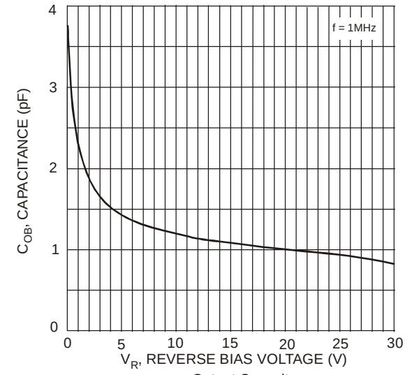
Fig.10 Output Capacitance
