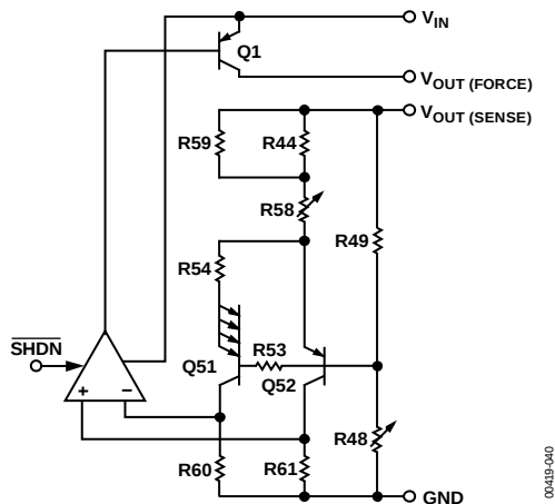
Figure 33. Simplified Schematic
