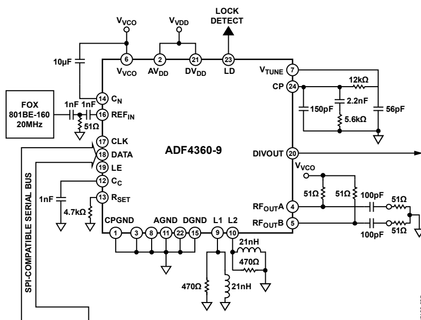
Figure 30.GSM Test Clock
