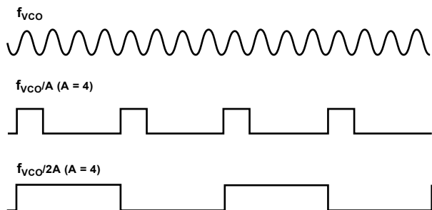
Figure 21. DIVOUT Waveforms
