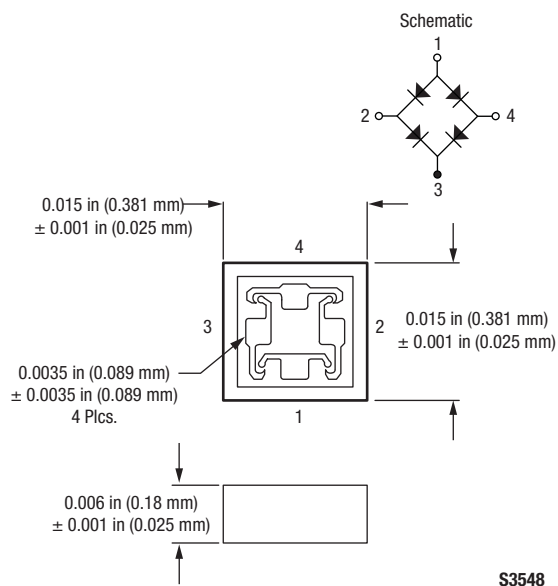
Figure 7. 551-004 Package Dimensions
