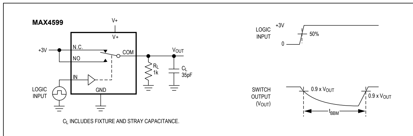
Figure 3. Break-Before-Make Interval
