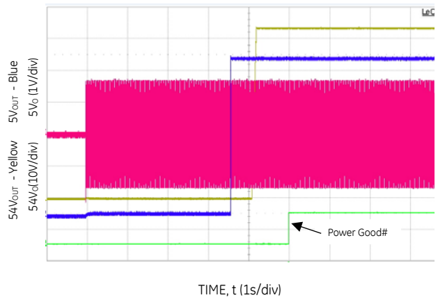
Figure 14. Turn-ON at full load V_{IN} = 230V_{AC} .
