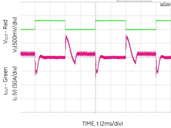
Figure 7. Transient response 54V DC load step 10 – 60%, Slew rate: 1A/μs, V IN = 230V AC
