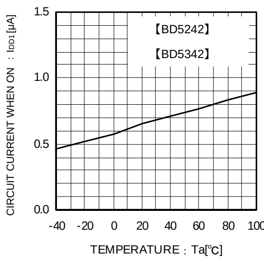
Fig.10 Circuit Current when ON
