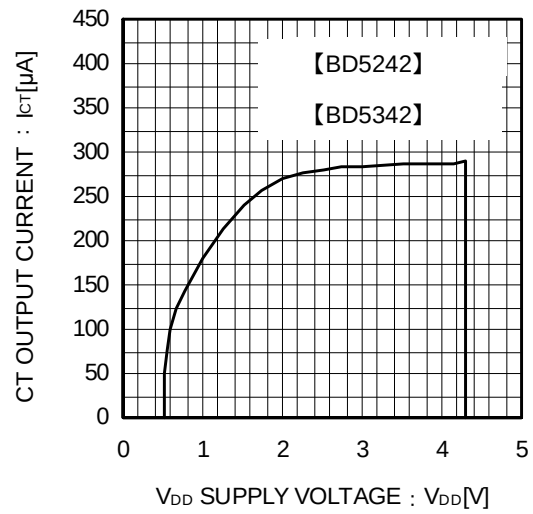
Fig.8 CT Terminal Current
