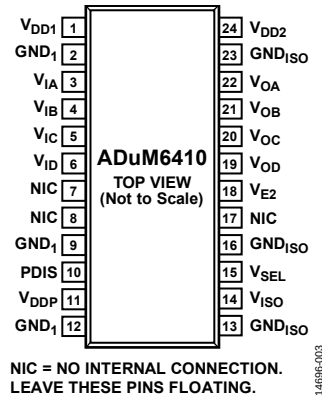
Figure 3. ADuM6410 Pin Configuration
