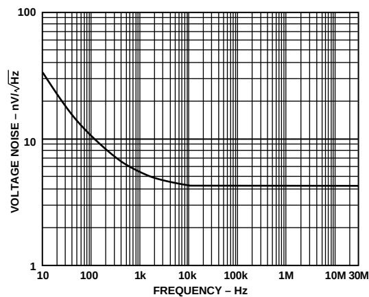
Figure 15. Voltage Noise vs. Frequency
