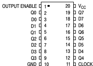
SOIC-20 DW SUFFIX CASE 751D
