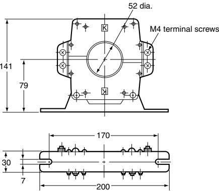
Indoor Separate-type Models OTG-CN52 (200 A)
