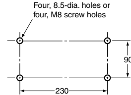
Mounting Hole Cutout Dimensions
