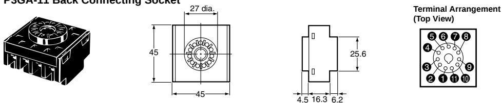
P3GA-11 Back Connecting Socket
