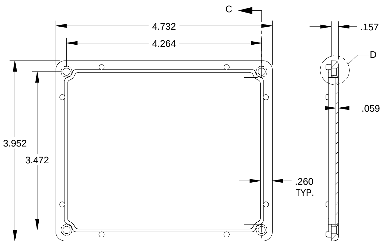
SECTION C-C
