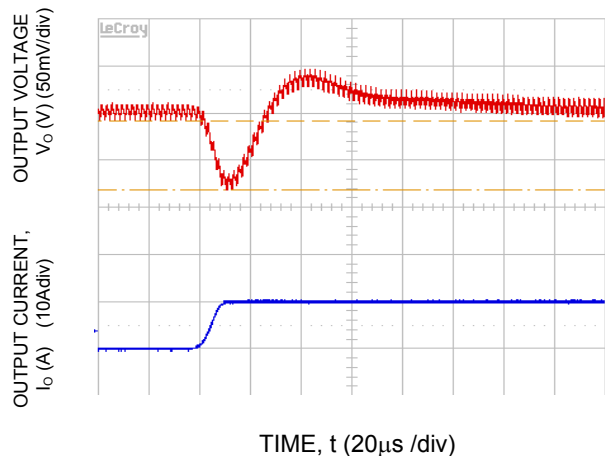
Fig-24. Transient Response to Dynamic Load Change from 50% to 100% at 12Vin, C out =5x47uF+1x330uF, CT tune =2200pF & RT tune =220ohms
