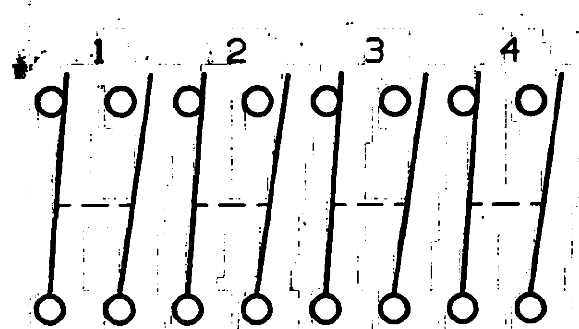
CIRCUIT DIAGRAM OF POSITIONS FOR DTS4SD
