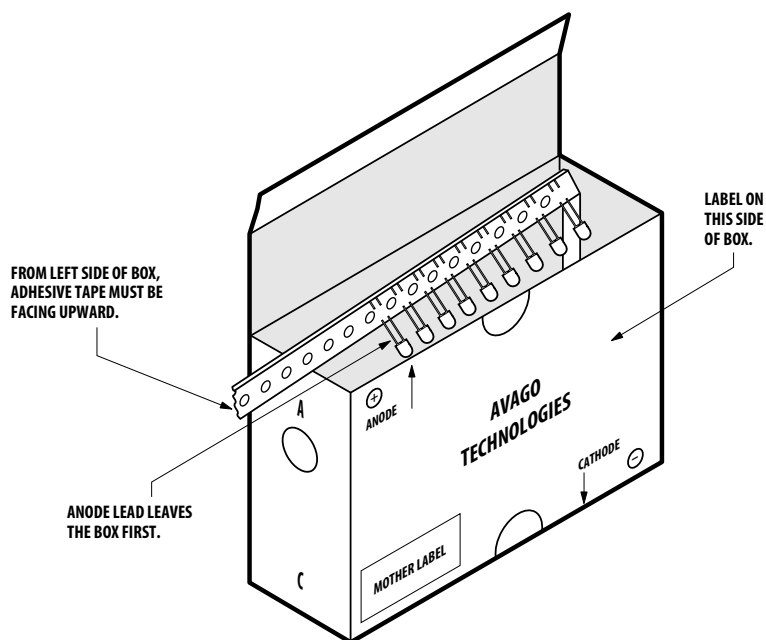
Figure 14: Packaging Box for Ammo Packs
