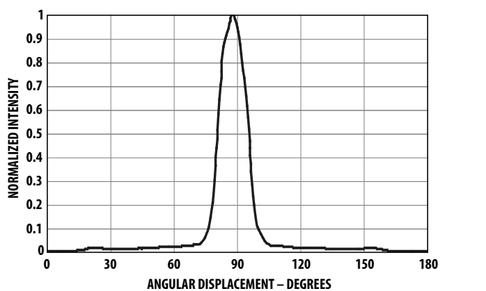
Figure 7: Representative Spatial Radiation Pattern for 15° Viewing Angle Lamps
