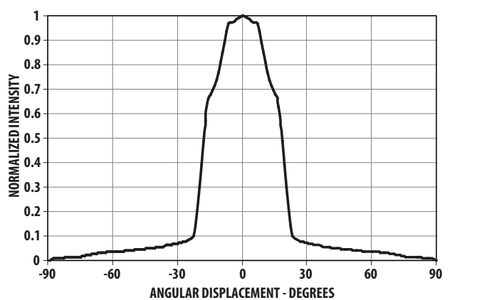
Figure 9: Representative Spatial Radiation Pattern for 30° Viewing Angle Lamps
