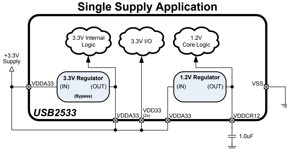
Figure 4.1 Power Connections
