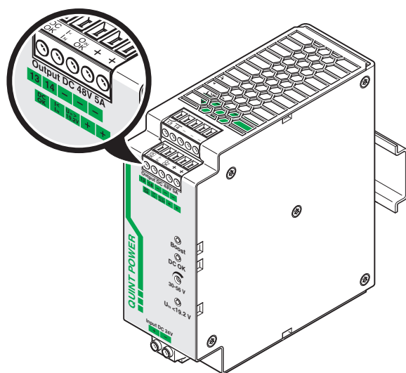
Figure 12 Signal outputs
