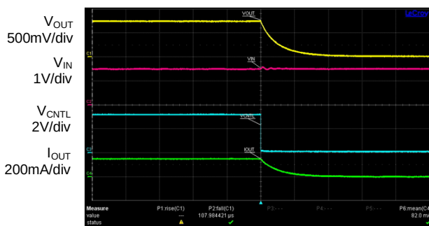
VCNTL Power Off ( C_{IN}=C_{OUT}=10\mu F , R_{LOAD}=5\Omega )
