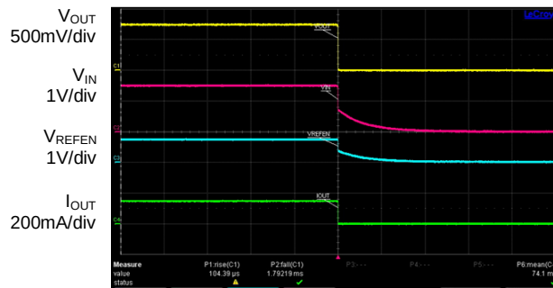
VIN Power Off ( C_{IN}=C_{OUT}=10\mu F , R_{LOAD}=5\Omega , V_{CNTL}=5V )
