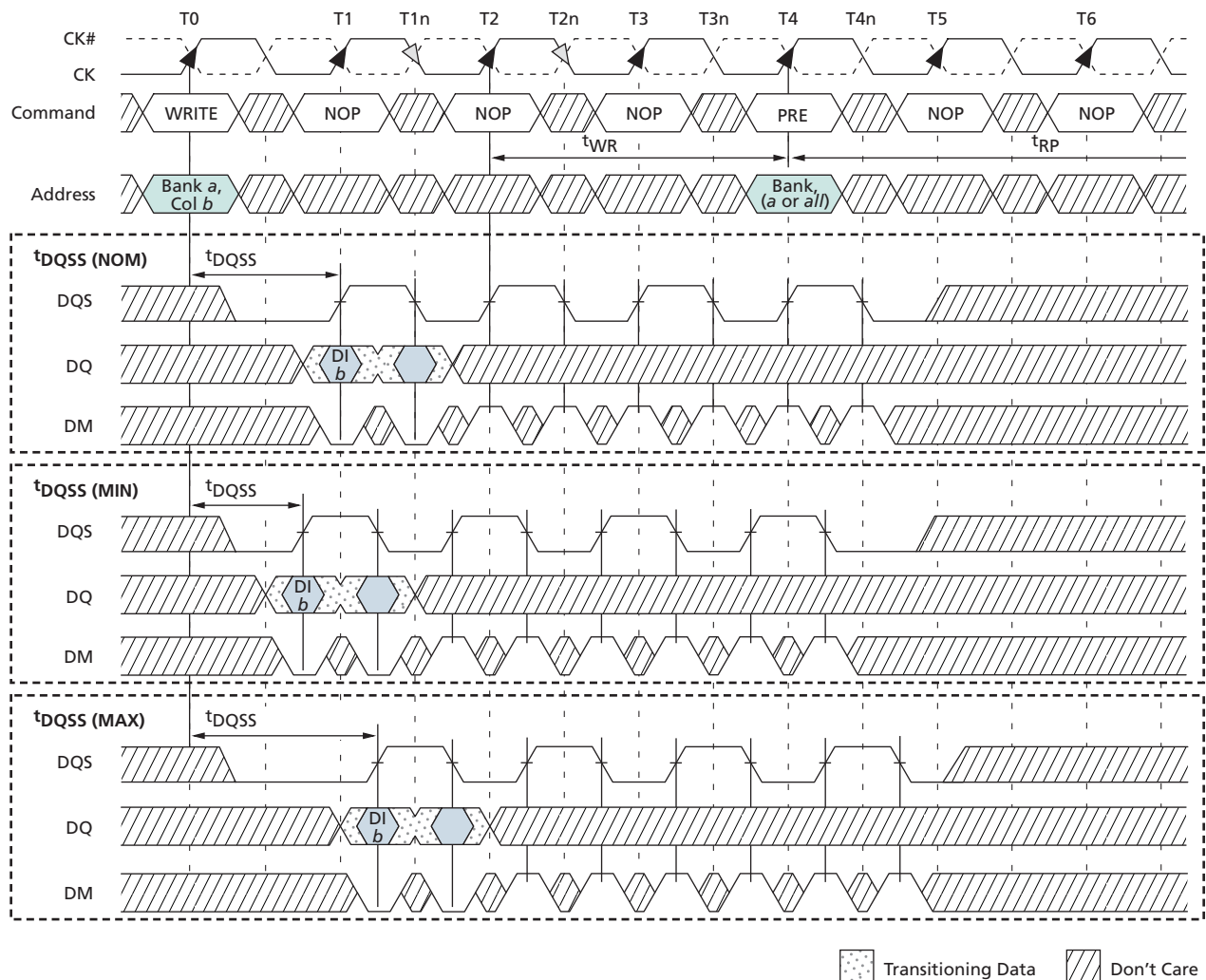
Figure 45: WRITE-to-PRECHARGE – Interrupting
