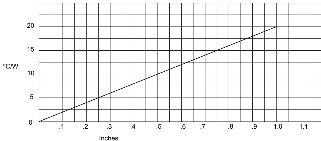
Figure 3 Typical Thermal Resistance versus Lead Length
