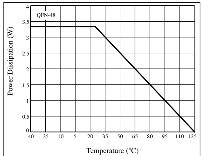
Figure 18 Dissipation Curve
