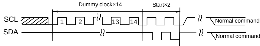
Figure 40-(a). The Case Of Dummy Clock×14 + START+START+ Command Input
