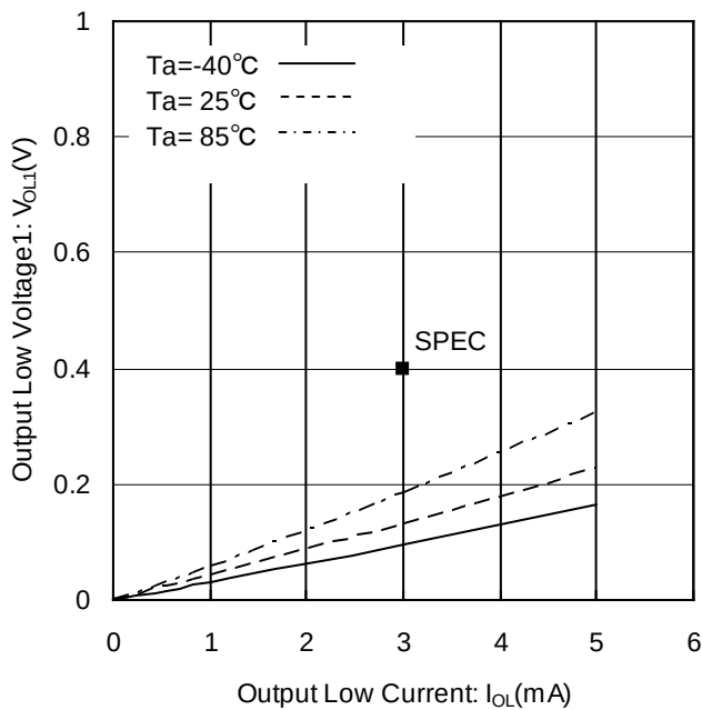
Figure 6. Output Low Voltage1 vs Output Low Current (V&lt;sub&gt;CC&lt;/sub&gt;=2.5V)
