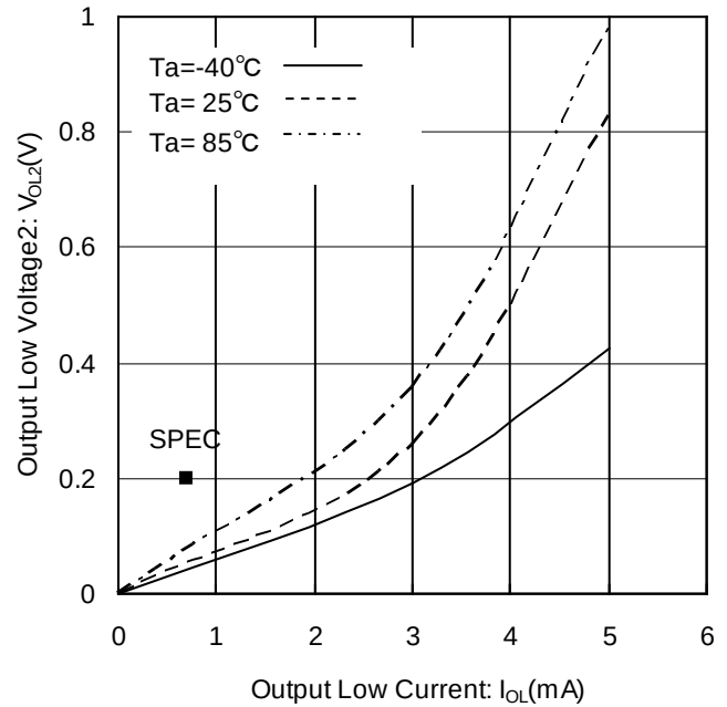
Figure 7. Output Low Voltage2 vs Output Low Current (V&lt;sub&gt;CC&lt;/sub&gt;=1.6V)
