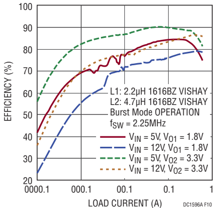
Figure 10. Efficiency
