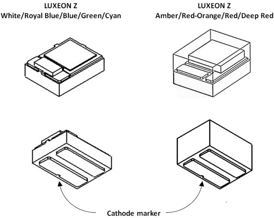
Figure 4. Pad configuration.
