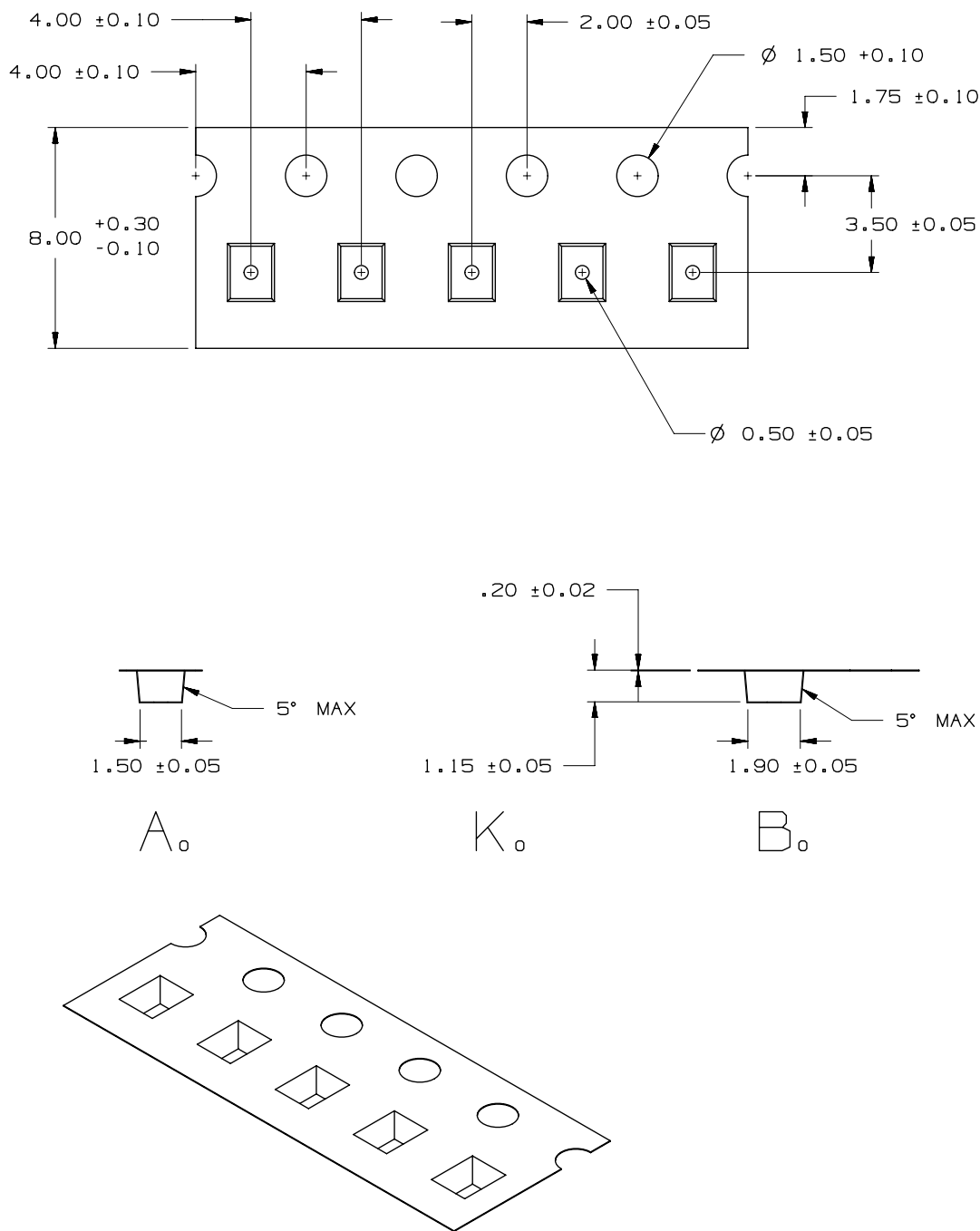
Figure 24. Emitter pocket tape packaging for LXZ1-PL01, LXZ1-PA01, LXZ1-PD01, LXZ1-PH01, LXZ1-PH02, LXZ1-PD02 and LXZ1-PL03.
