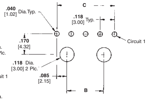
Recommended PC Board Layout 4-12 Position*
