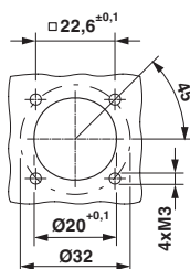
Dimensional drawing
