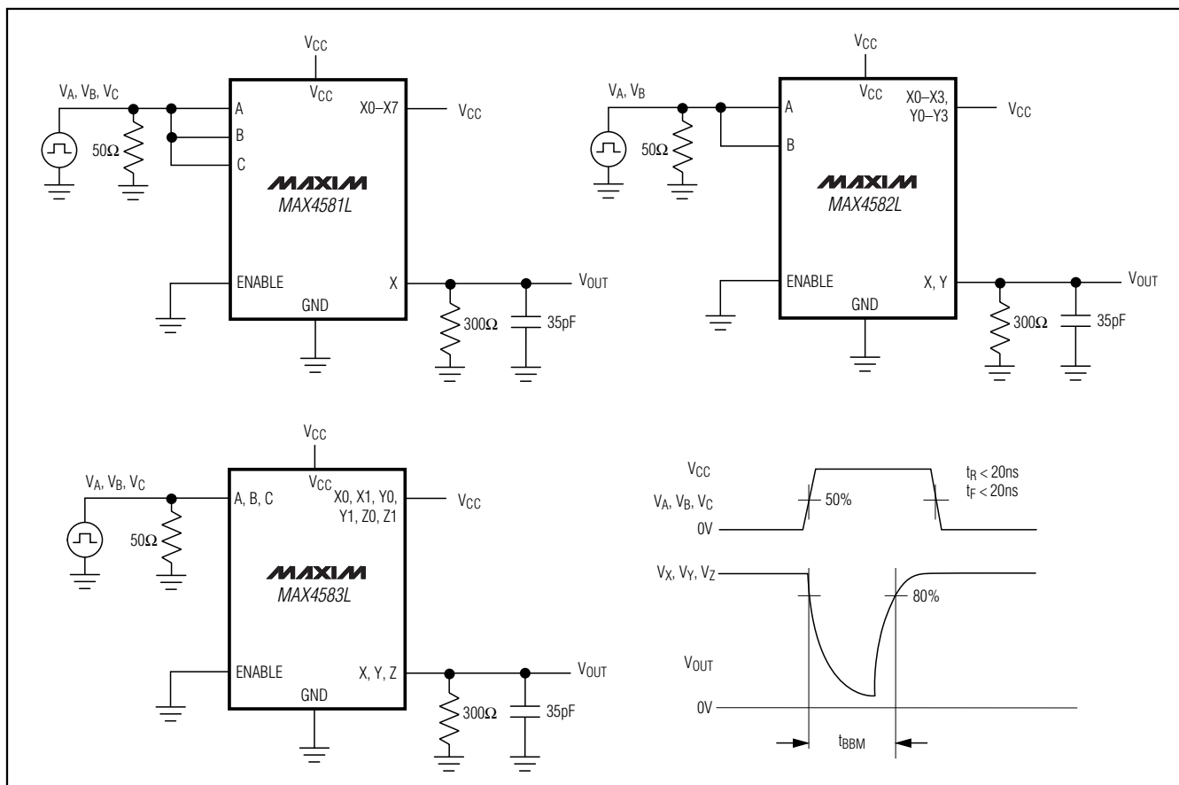
Figure 3. Break-Before-Make Interval
