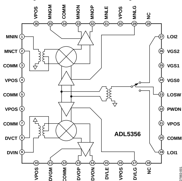
Figure 52. Simplified Schematic
