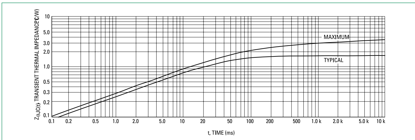
Figure 10. Thermal Response
