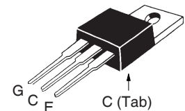
TO-220 (IXYP)
