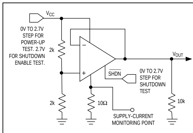
Figure 10. Power-Up/Shutdown Test Circuit
