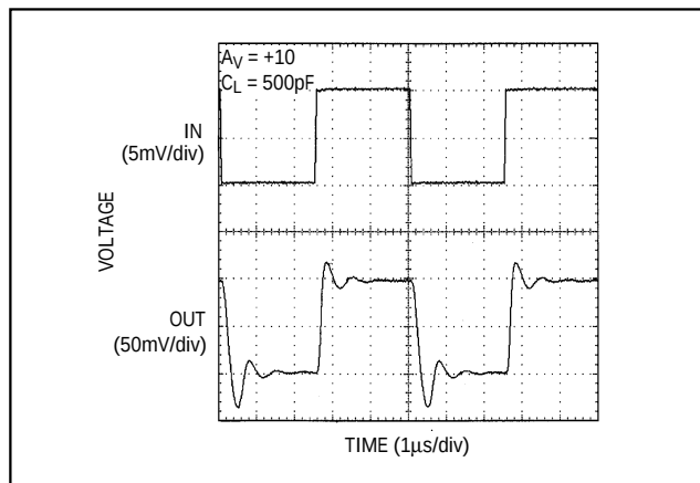
Figure 6. MAX4124/25/28 Small-Signal Transient Response with Capacitive Load
