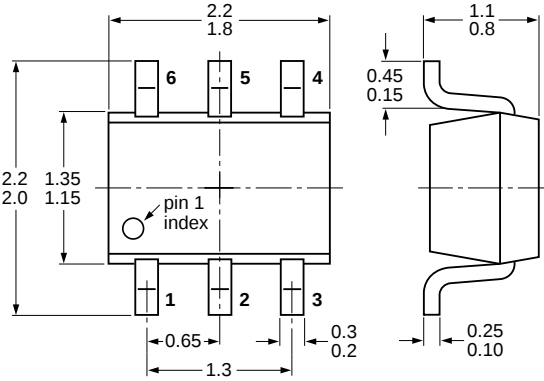
Fig 11. Package outline PUMH13 (SOT363)
