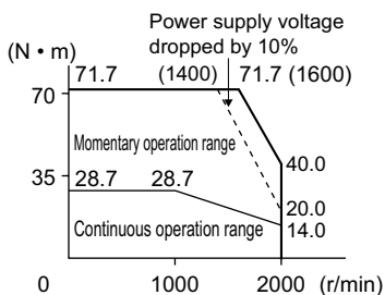
R88M-K3K010(H/T/F/C)-□ (3 kW)
