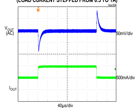
MAXM17624 LOAD TRANSIENT RESPONSE V_{IN} = 5V , V_{OUT} = 3.3V , PWM MODE (LOAD CURRENT STEPPED FROM 0.5 TO 1A)
