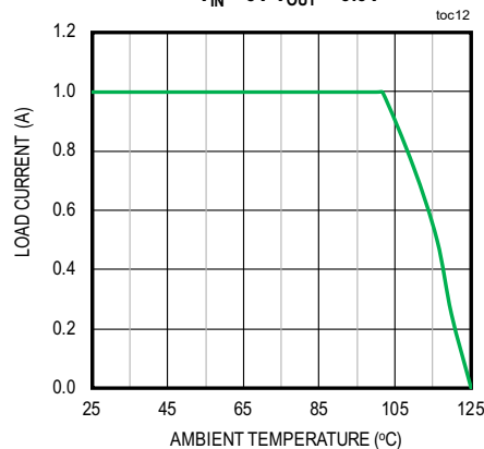
MAXM17624 OUTPUT CURRENT vs. AMBIENT TEMPERATURE
