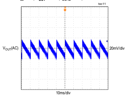
MAXM17624 OUTPUT VOLTAGE RIPPLE
