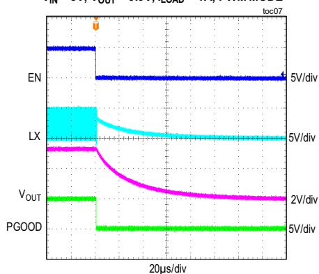
MAXM17624 SHUTDOWN THROUGH ENABLE
