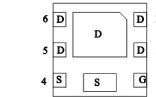
Pin Out Bottom View
