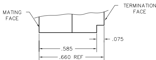
DETAIL A
