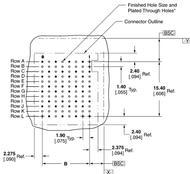
* Finished Hole Diameter = 0.46 \pm^{+0.05}_{-0.01} [0.18 \pm^{+0.002}_{-0.001} ] Drilled Hole Diameter = 0.55 \pm^{+0.02}_{-0.01} [0.22 \pm^{+0.001}_{-0.001} ] Copper Thickness = 0.038 \pm^{+0.013}_{-0.005} [0.015 \pm^{+0.005}_{-0.005} ] Tin-Lead Thickness = 0.008 \pm^{+0.004}_{-0.003} [0.003 \pm^{+0.002}_{-0.002} ] Finishes other than Tin-Lead. See Appl. Spec. 114-13202
